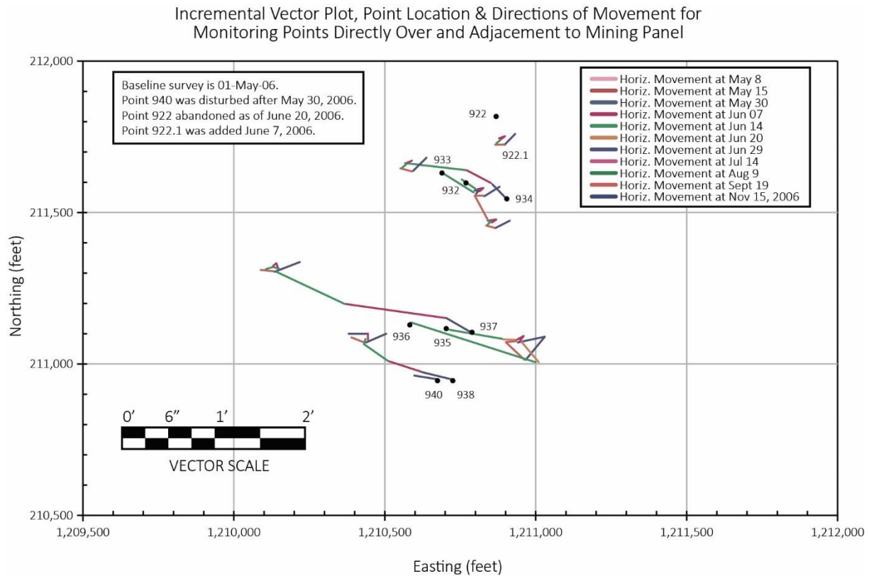
Figure 26. Ryerson Dam control site monitoring data (source: Hebblewhite & Gray, 2014) (Numbers refer to monitoring stations as marked in Figure 25)
