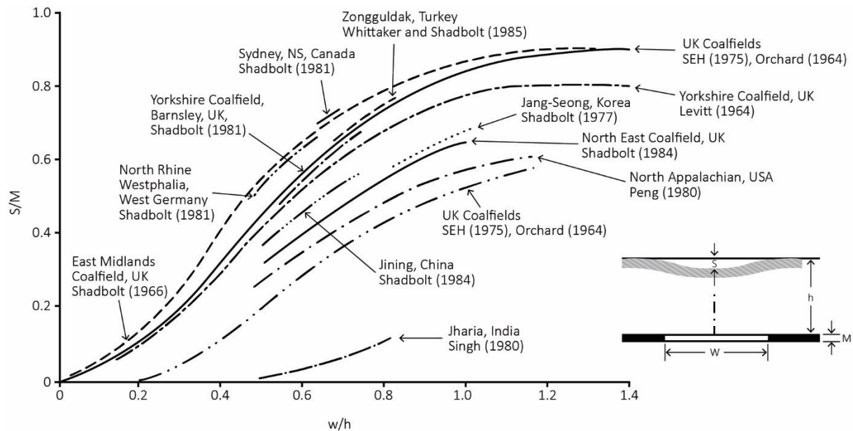
Figure 19. International maximum subsidence prediction curves (source: NSW Dept of Planning, 2008; adapted from Whittaker and Reddish, 1989)
