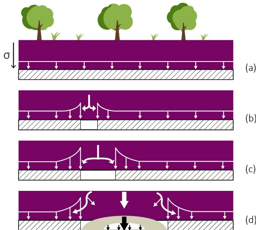
Figure 12. Abutment stresses associated with excavations and increasing spans (source: UNSW Sydney, 2014)
