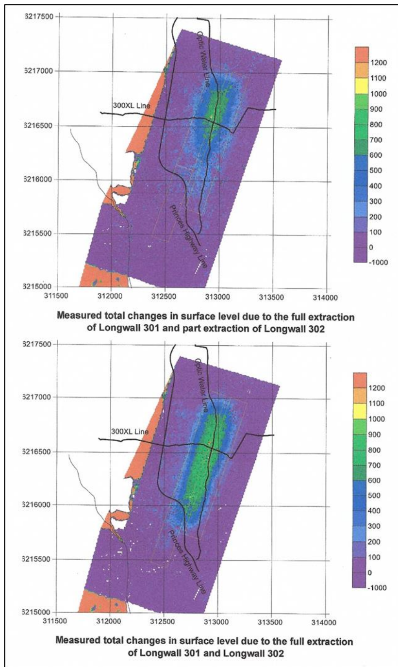
Figure 32. LiDAR subsidence survey results over Metropolitan Colliery (source: Hebblewhite et al, 2019)
