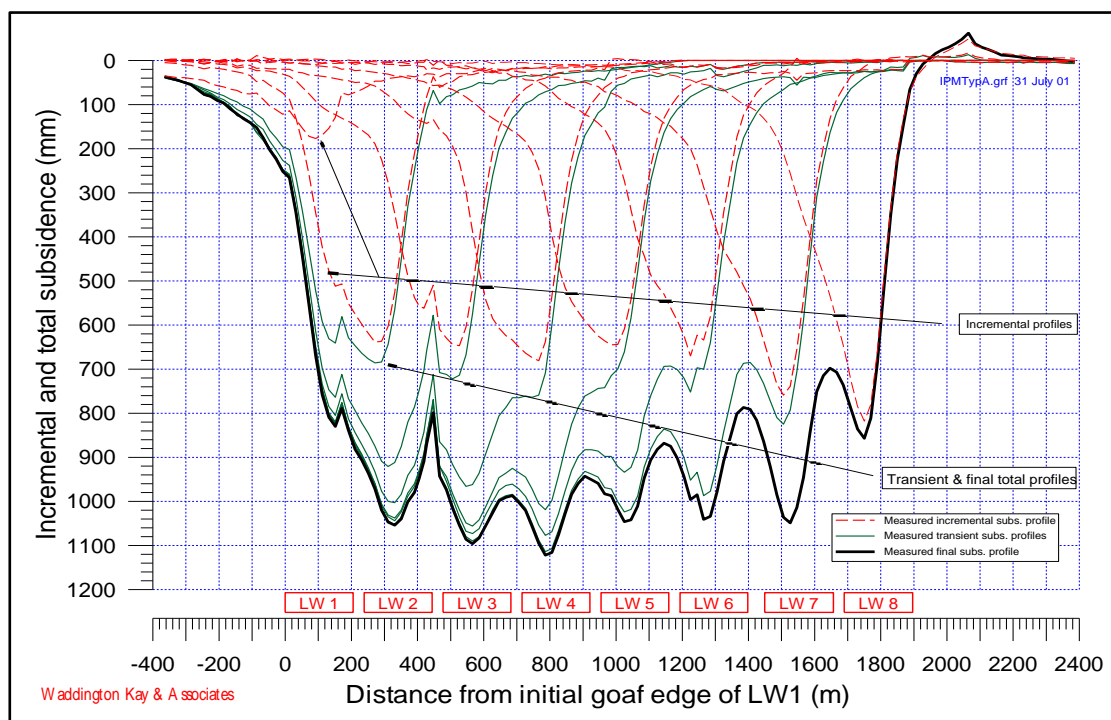
Figure 27. Development of incremental and total subsidence over multiple panels
