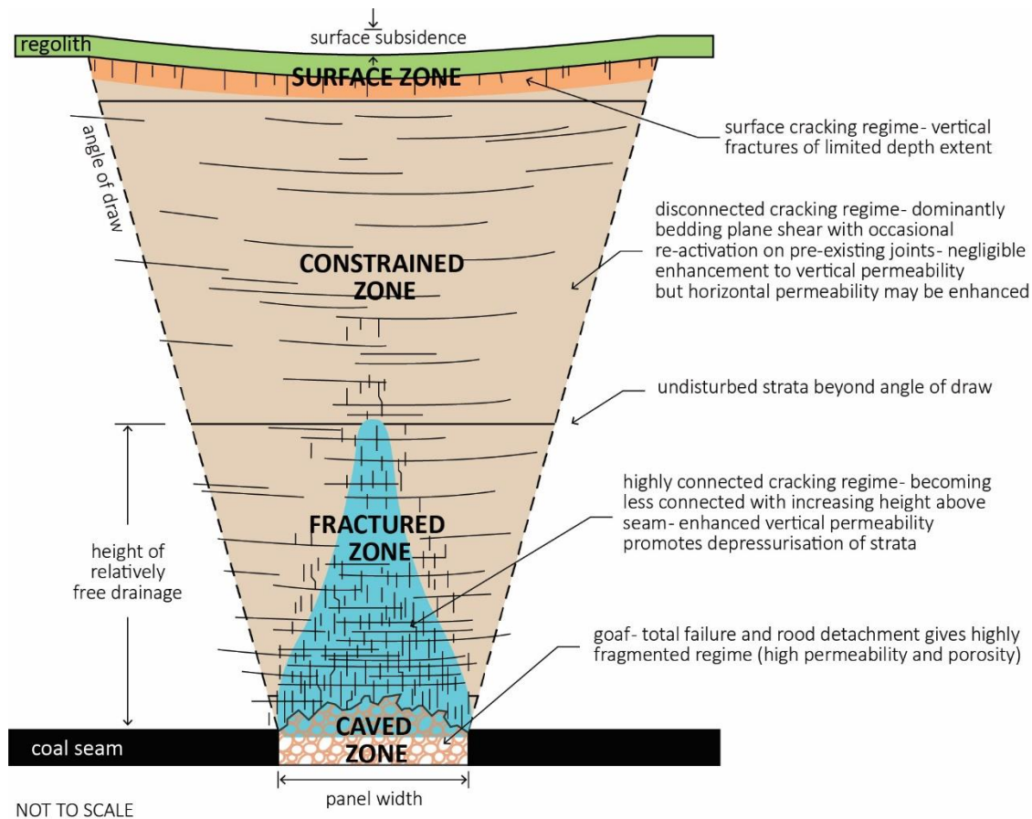
Figure 31. Conceptual model of fracture zones above a caved mining extraction panel (source: NSW Dept of Planning, 2008, after Mackie)
