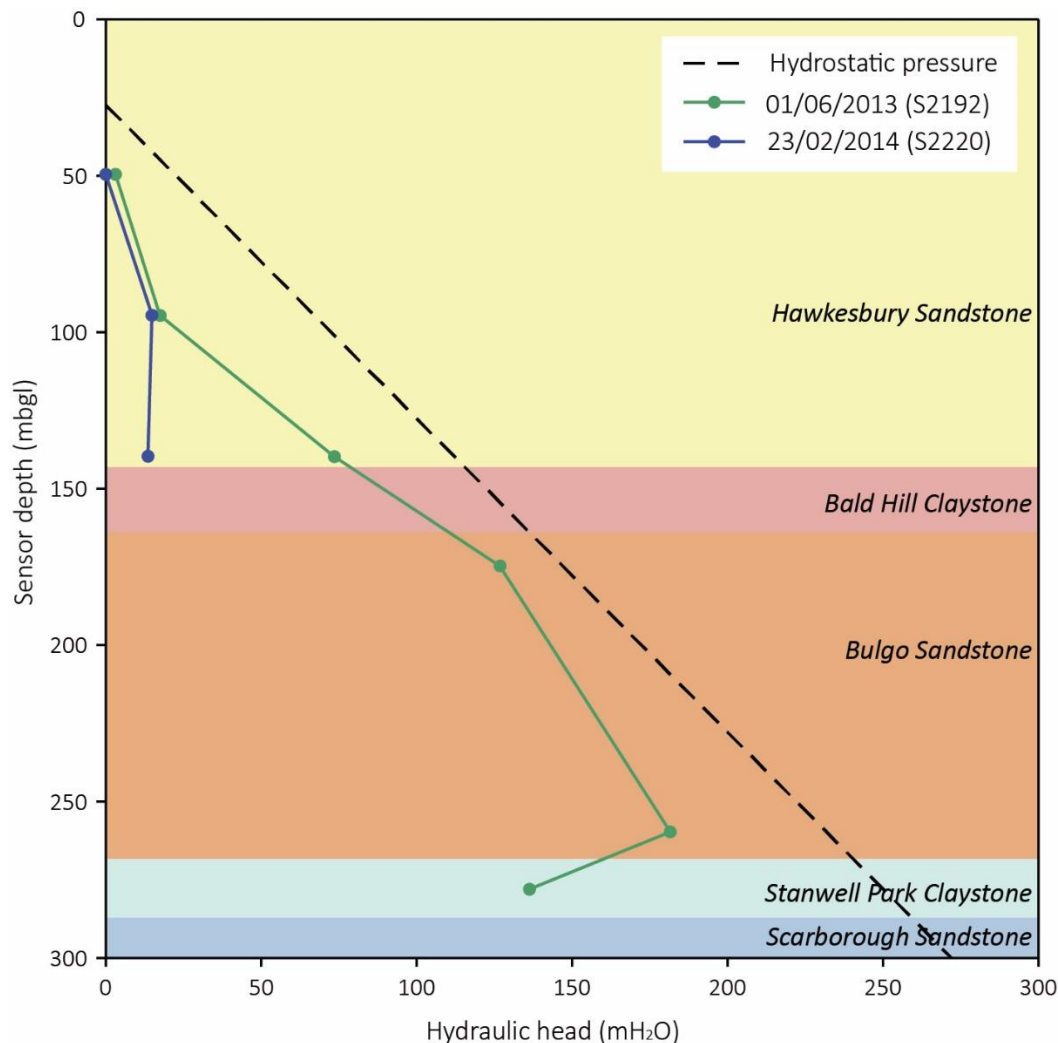
Figure 39. Example of height of depressurisation detection above mining (source: Hebblewhite, 2019)
