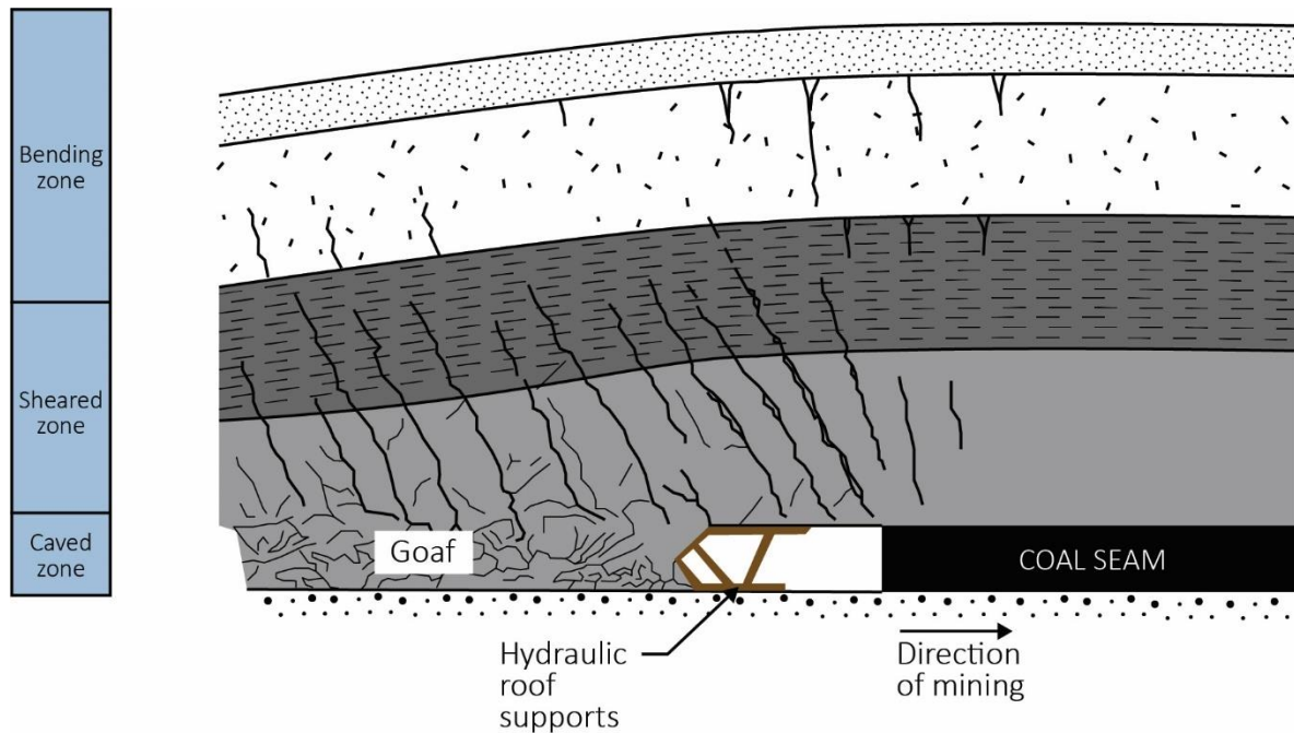
Figure 9. Typical caving and overburden response to undermining, behind the longwall face (source: adapted from National Coal Board, 1966)
