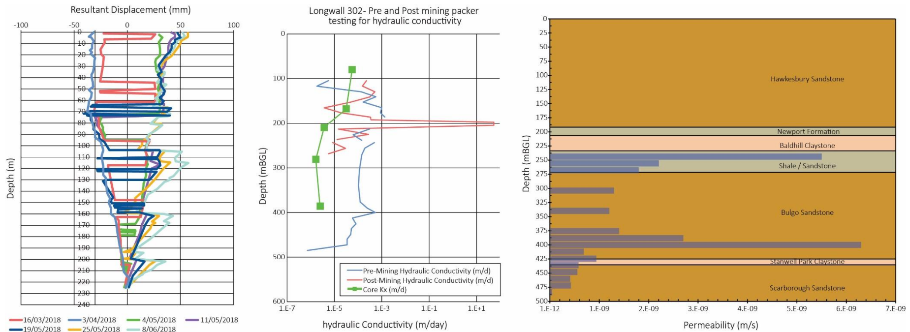
Figure 40. Example of combined bedding plane shear and hydraulic conductivity results (source: Hebblewhite et al., 2019)
