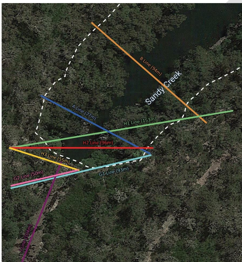
Figure 34. High-precision closure line surveys to monitor valley closure at Sandy Creek Waterfall (source: Walsh et al., 2014) (Each coloured line indicates a line-of-sight high-precision survey line, as marked).
