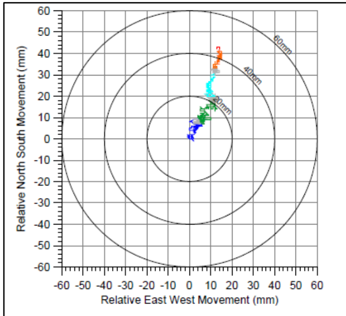
Figure 33. Example of GNSS monitoring results (colour-coded for each successive longwall) (source: Hebblewhite et al, 2019)
