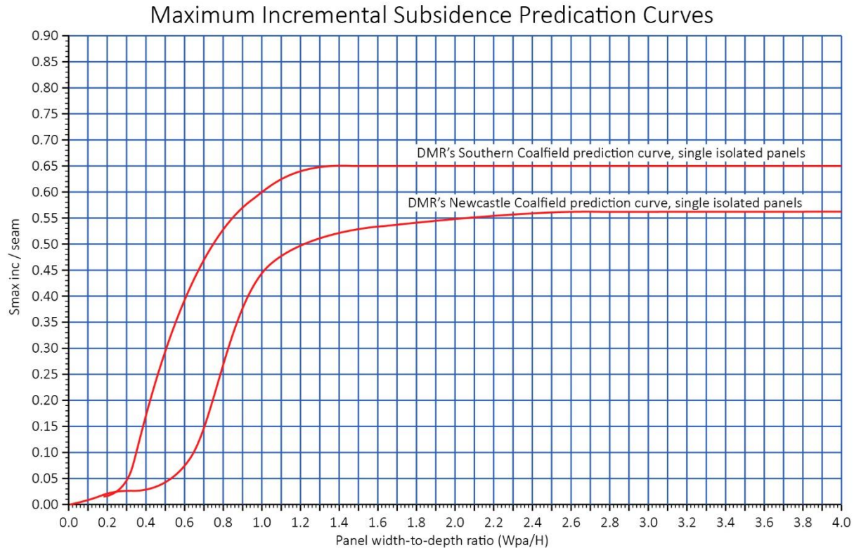
Figure 18. Maximum incremental subsidence relative to panel width and depth
