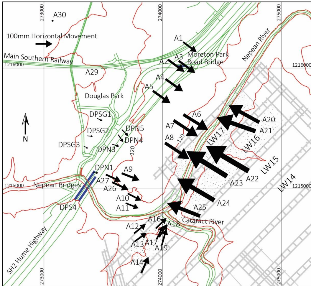
Figure 24. Horizontal movement above Tower Colliery longwalls (source: Hebblewhite, 2001) (Arrows are positioned centrally over each monitoring station. Arrow size indicates magnitude of movement, relative to scale in top left of diagram).
