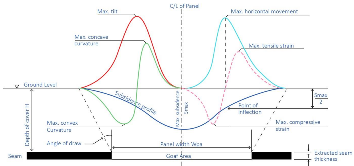
Figure 16. Conventional subsidence profile
