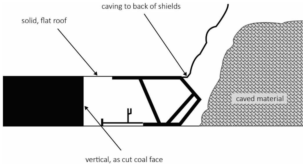
Figure 8. Idealised longwall face and caving conditions
