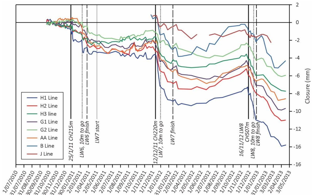
Figure 35. High precision closure results for valley closure at Sandy Creek Waterfall
