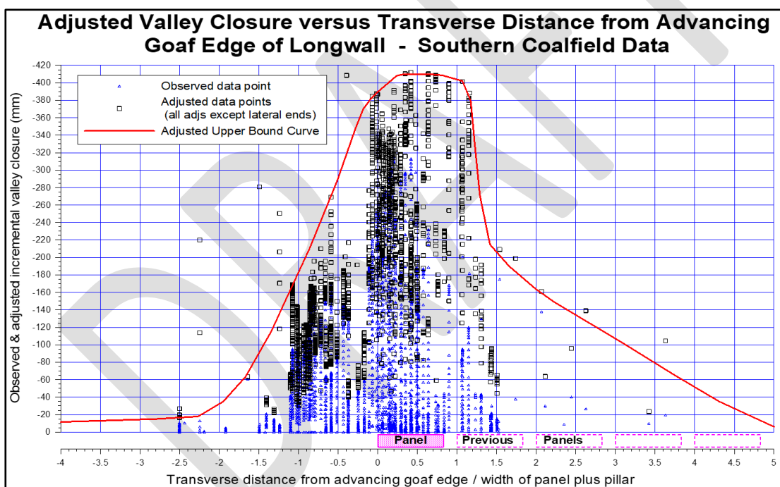
Figure 22. Southern Coalfield valley closure data (source: MSEC, 2014)
