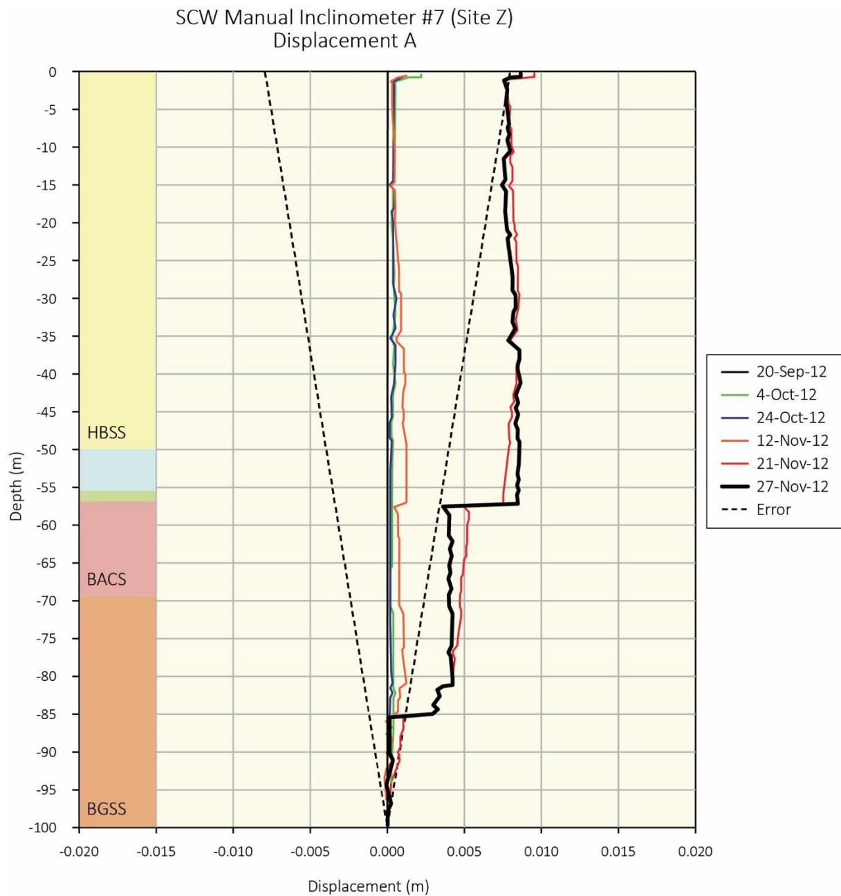
Figure 37. Borehole inclinometer results for detecting bedding plane shear (source: Walsh et al., 2014)
