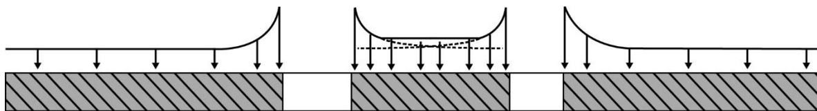
Figure 14. Abutment stresses associated with excavations and increasing spans
