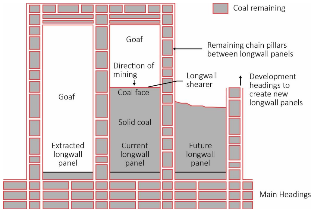
Figure 6. Typical longwall mining layout (source: UNSW Sydney, 2014)
