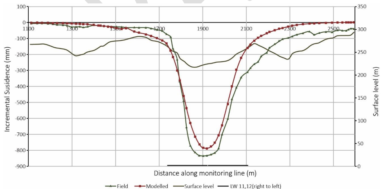
Figure 29. Prediction of subsidence using UDEC modelling (source: Zhang et al., 2014)
