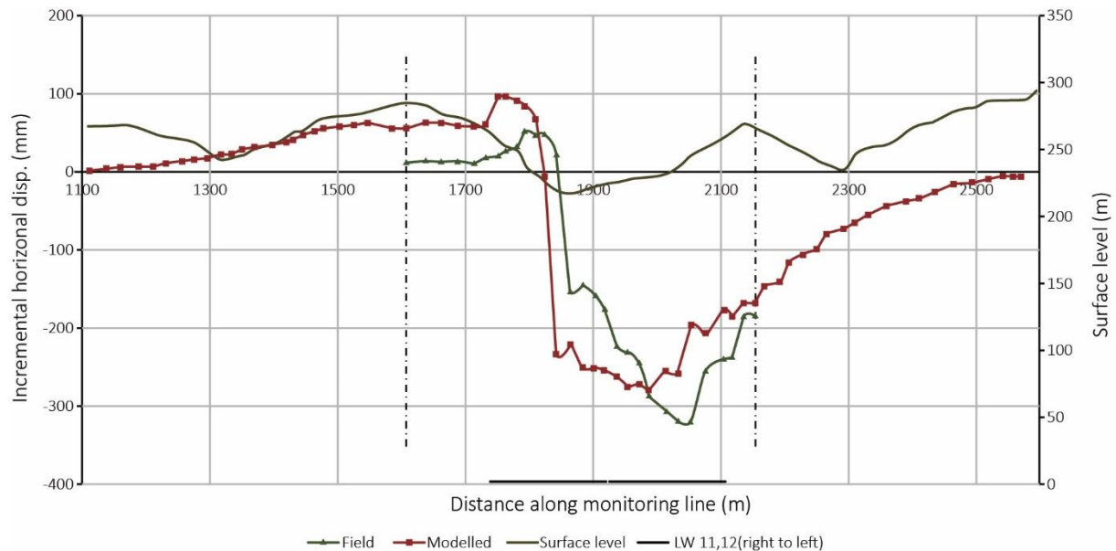
Figure 30. Prediction of horizontal displacement using UDEC modelling (source: Zhang et al., 2014)
