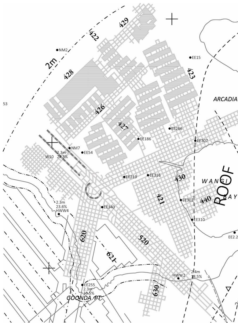
Figure 3. An example of a typical bord and pillar first workings mine layout (source: Hebblewhite, 2022b)
