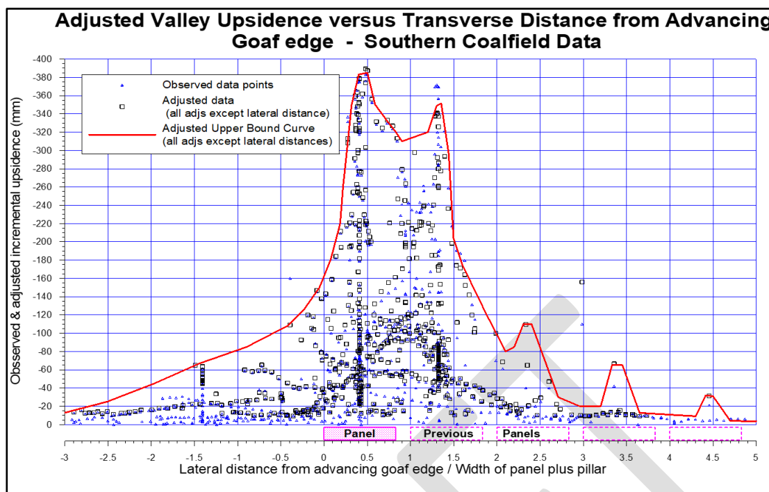
Figure 23. Southern Coalfield valley upside data (source: MSEC, 2014)
