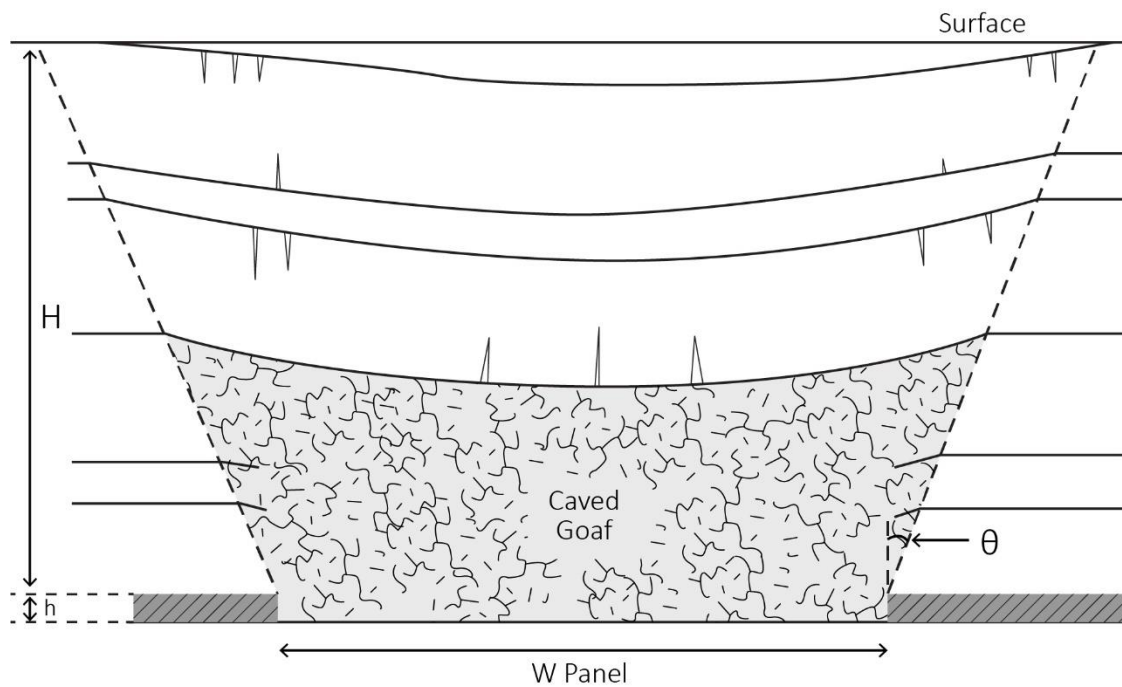
Figure 13. Caving or sag subsidence
