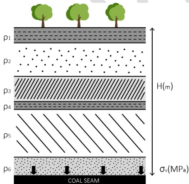
Figure 10. Pre-mining vertical stress at depth
