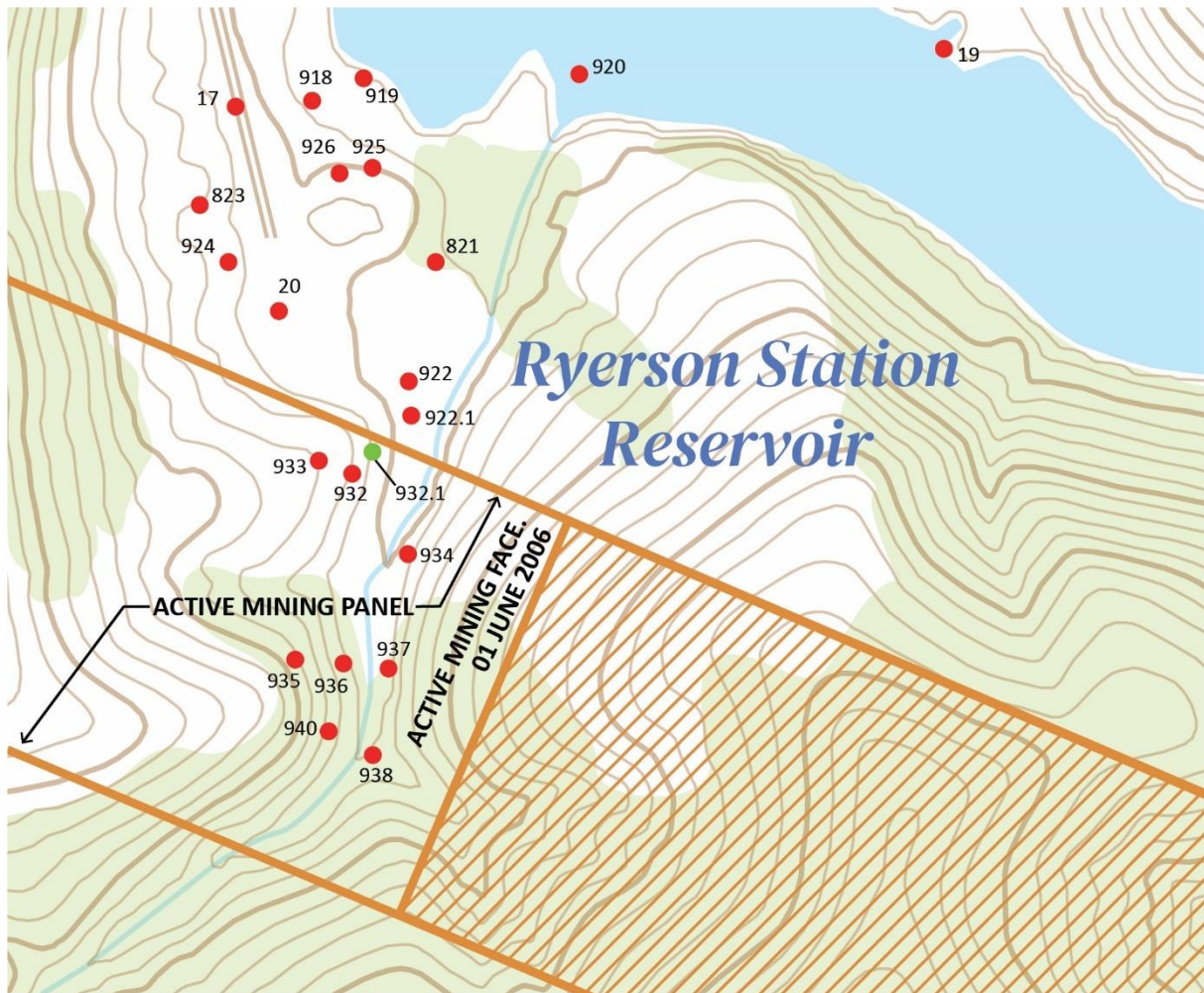
Figure 25. Ryerson Dam investigation site, Pennsylvania (source: Hebblewhite & Gray, 2014) (Numbered subsidence monitoring stations marked with a red dot and station number).
