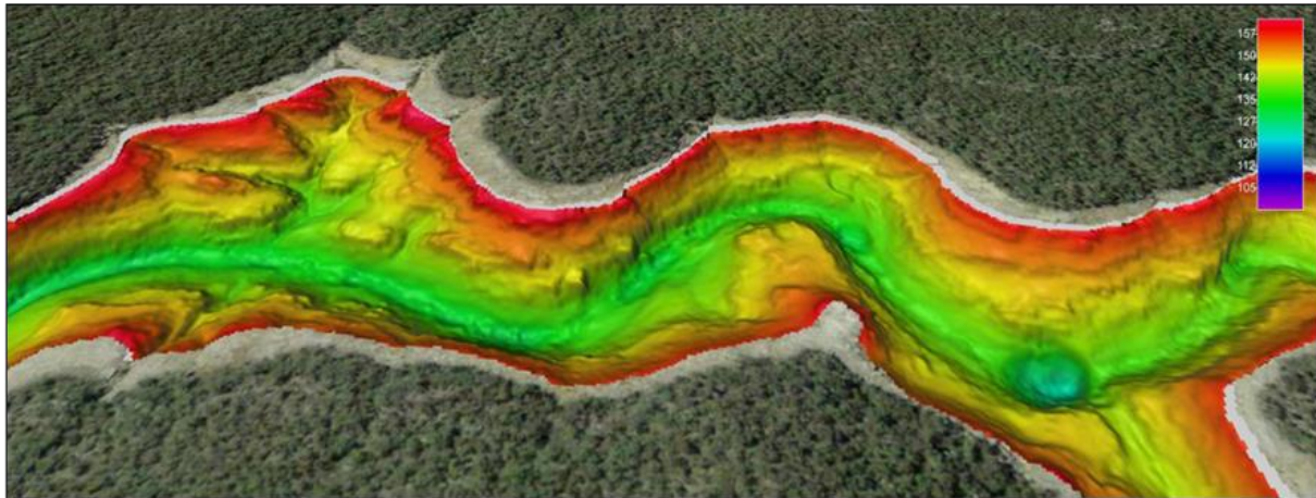
Figure 36. Bathymetric survey results showing 3D image of reservoir floor for Waratah Rivulet. (Coloured levels are noted in mAHd). (Source: Hebblewhite et al., 2017 after Ramsay et al., 2014)
