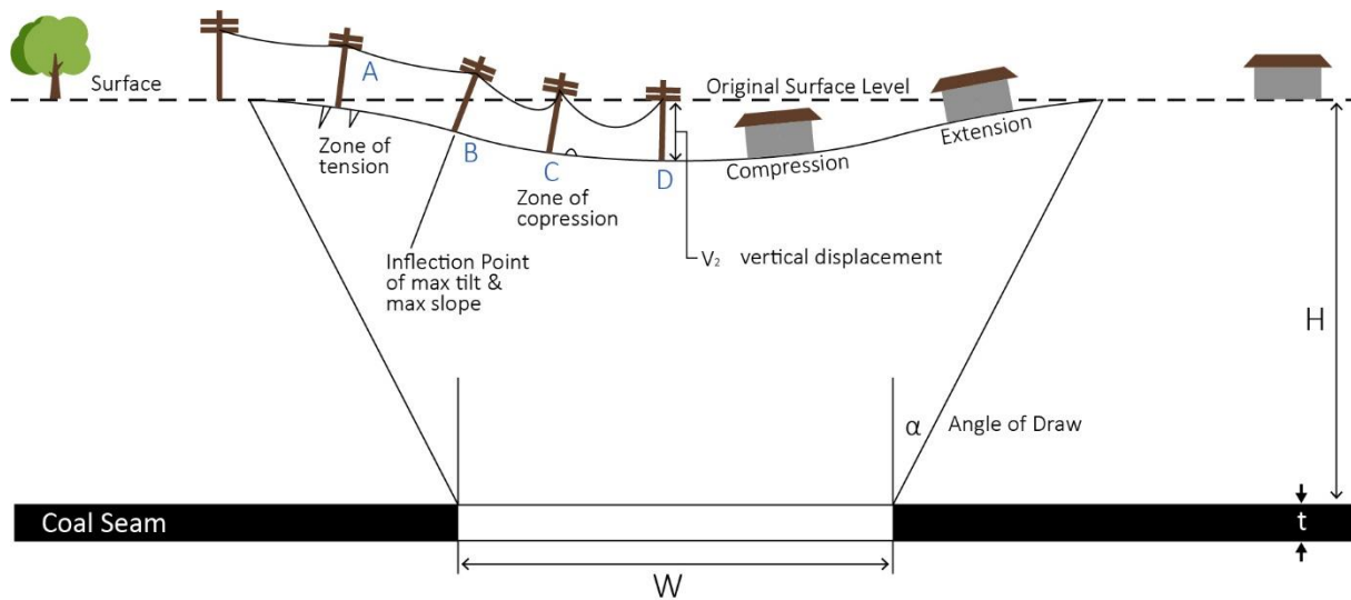
Figure 17. Surface response to subsidence – (exaggerated vertical scale)
