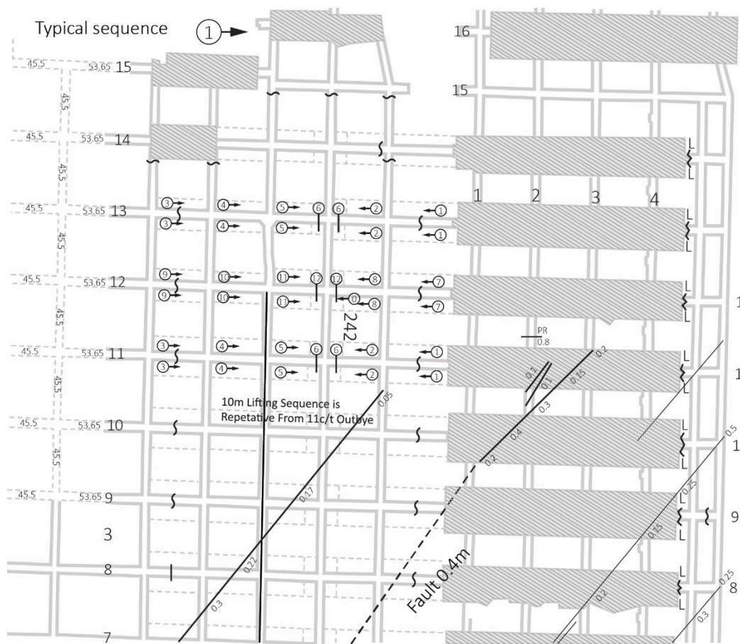
Figure 4. An example of a partial extraction mine layout – rib brushing (source: Hebblewhite, 2022b)
