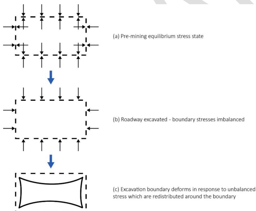
Figure 11. Vertical section through an excavation showing the stages of response of rock to disturbed equilibrium
