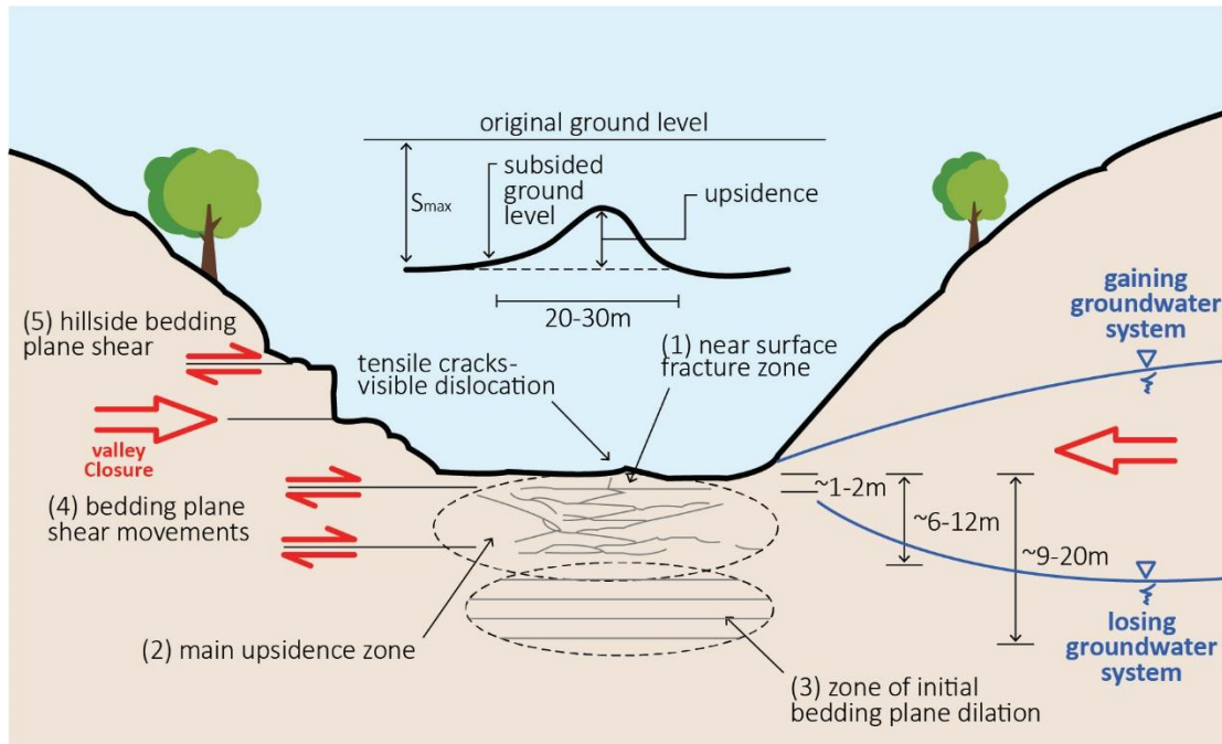
Figure 20. Sketch of conceptual mechanism for valley closure and upsidence (source: Mills, 2008)
